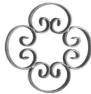
Art. 5A08 Ø 210 mm ▧ 16 x 4mm
