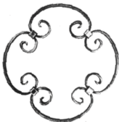
Art. 10A07 \sphericalangle 16 x 4 mm Art. 10A08 \sphericalangle 20 x 4 mm Art. 10A09 \sphericalangle 20 x 6 mm \phi 250 mm
