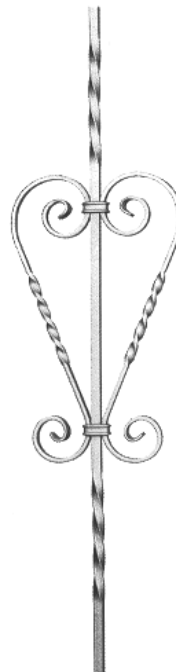
Art. 37A17 \phi 12 \square 12 \times 6 \text{ mm} Art. 37A18 \phi 14 \square 14 \times 6 \text{ mm} 220 x 900 mm
