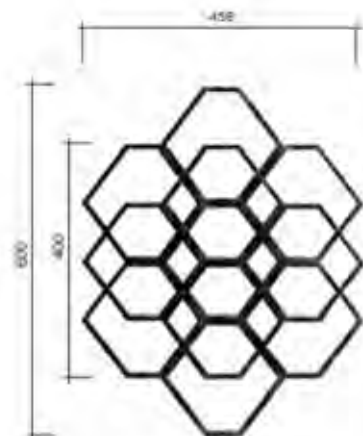
Art. 314A06 \varnothing 8 + \sphericalangle 16 \times 8 \text{ mm} H 600 mm L 458 mm
