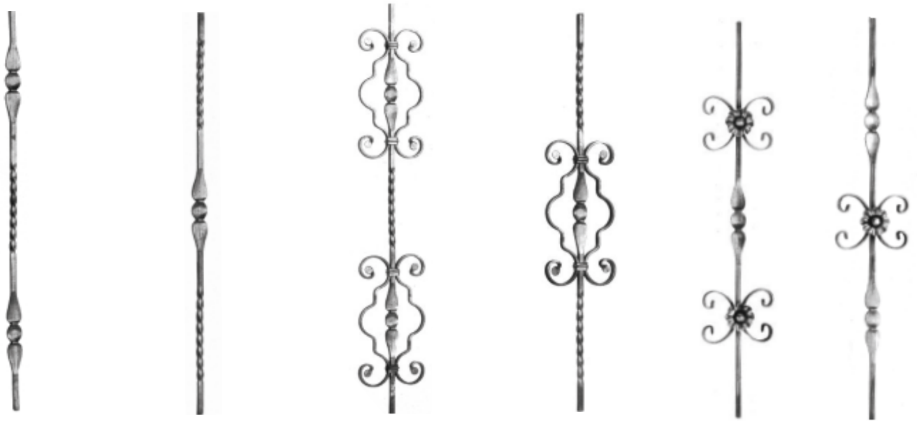
Art.115A01 H 900 Art.115A07 H 900 Art.115A13 H 900 Art.115A19 H 900 Art.115A25 Art.115A27 Art.115A02 H1200 Art.115A08 H1200 Art.115A14 H1200 Art.115A20 H1200 ∅ 12 mm ∅ 12 mm ∅ 12x6 mm ∅ 12x6 mm ∅ 12x6 mm ∅ 12x6 mm Art.115A26 Art.115A28 Art.115A03 H 900 Art.115A09 H 900 Art.115A15 H 900 Art.115A21 H 900 ∅ 14 mm ∅ 14 mm Art.115A04 H1200 Art.115A10 H1200 Art.115A16 H1200 Art.115A22 H1200 155x900mm 155x900mm ∅ 12 mm ∅ 12 mm ∅ 12 mm ∅ 12 mm Art.115A05 H 900 Art.115A11 H 900 Art.115A17 H 900 Art.115A23 H 900 Art.115A06 H1200 Art.115A12 H1200 Art.115A18 H1200 Art.115A24 H1200 ∅ 14 mm ∅ 14 mm ∅ 14 mm ∅ 14 mm
