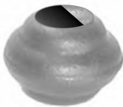
Art. 177B04 Ø 35 H 25 Foro Ø 12 Art. 177B05 Ø 37 H 35 Foro Ø 14 Art. 177B06 Ø 37 H 35 Foro Ø 16 Art. 177B07 Ø 55 H 35 Foro Ø 18 Art. 177B08 Ø 55 H 35 Foro Ø 20 Art. 177B09 Ø 55 H 35 Foro Ø 22 Art. 177B10 Ø 55 H 35 Foro Ø 25 Art. 177B11 Ø 55 H 35 Foro Ø 27 Art. 177B12 Ø 55 H 35 Foro Ø 30 Art. 177B13 Ø 70 H 35 Foro Ø 30 Art. 177B14 Ø 70 H 35 Foro Ø 35 Art. 177B15 Ø 70 H 35 Foro Ø 40 Art. 177B16 Ø 70 H 35 Foro Ø 42
