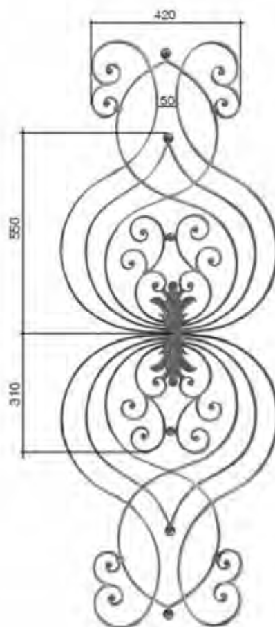
Art. 306A06 ▧ 14 x 8 mm H 1600 L 600 mm
