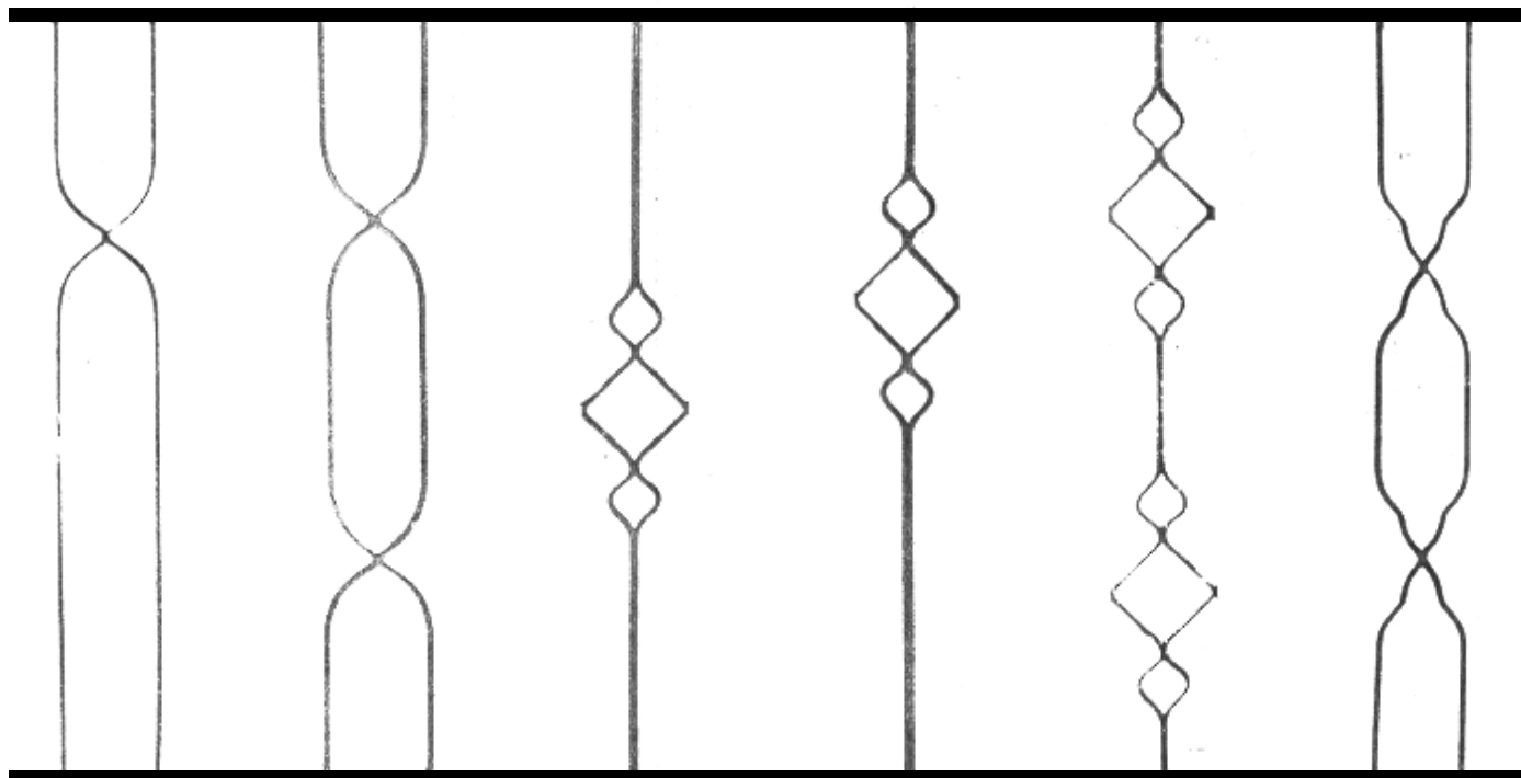
50A01 ▧ 20x4 50A02 ▧ 25x4 H 800 mm
