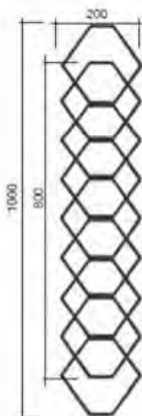
Art. 314A05 \varnothing 8 + \sphericalangle 16 \times 8 \text{ mm} H 1000 mm L 200 mm
