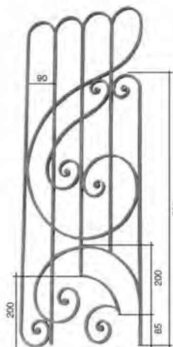
Art. 313A07 Ø14 x 8 mm H 1000 mm L 385 mm
